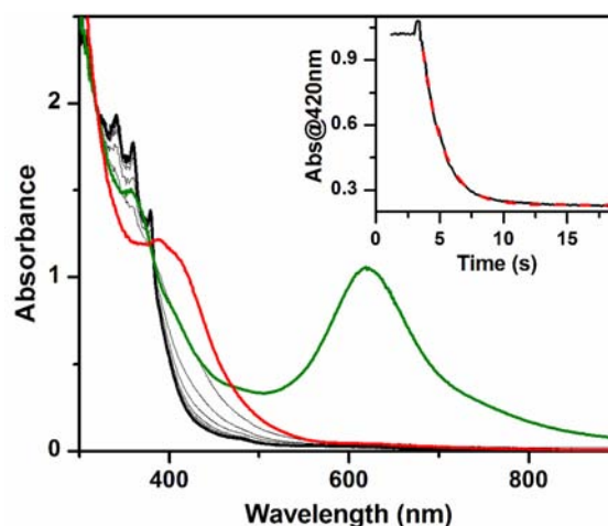
Figure 1. UV-vis spectra of complexes 1 (green line, 0.2 mM) and 1 -F (red line) obtained upon addition of \text{Bu}_4\text{NF} to the solution of 1 . Additional gray lines show the spectroscopic changes during the reaction of 1 -F with 2.0 mM DHA until the reaction is complete (black line). Inset: time trace at 420 nm (black solid line) together with the fit (red dashed line) using a first-order model. Conditions: in 3:1 \text{CH}_2\text{Cl}_2 -MeCN under Ar at -80 °C.
